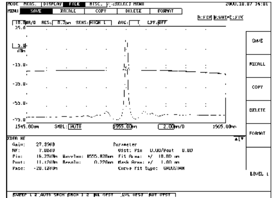
Example of measurement result. (Gain,NF)
