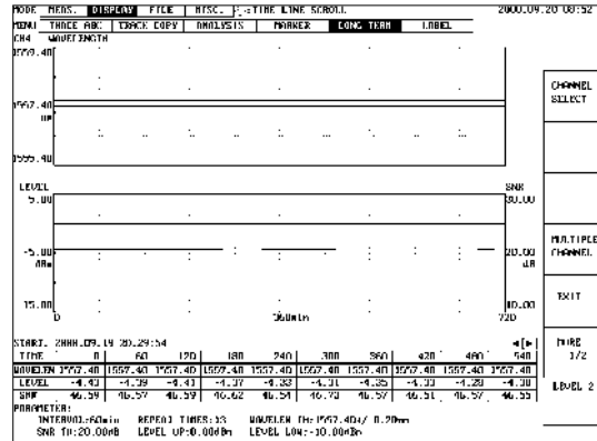
Long-term function (Example of single channel display)
